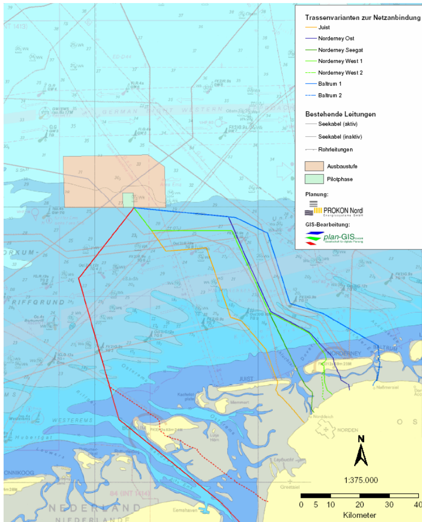
Figure 4-2: Seven different proposals for the sea cable routes (Source: Prokon Nord).
