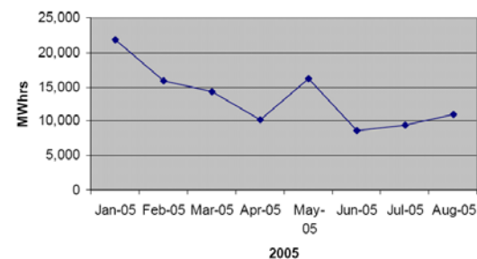
Figure 9-9: Availability and Generation of Electricity at Scroby Sands Wind Farm 132 .
