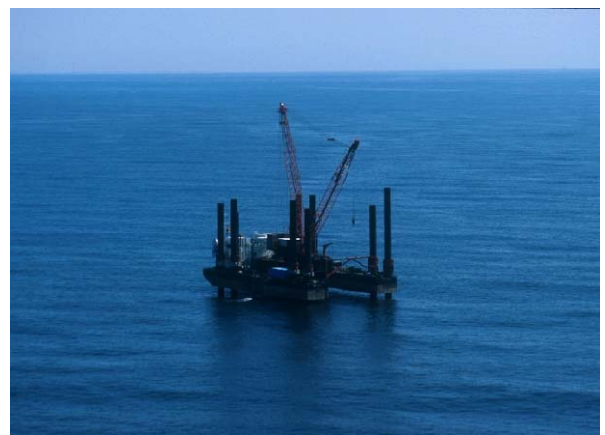
Figure 5-4: Drilling and conic penetration test with a platform from Mohiba.
